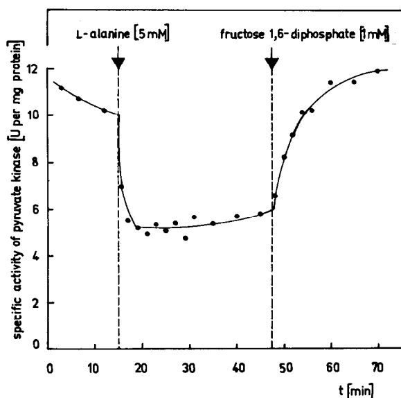
Fig. 3. Inhibition and reactivation of pyruvate kinase by L-alanine and fructose 1,6-diphosphate. Experimental: The enzyme was diluted in 40 mM Tris buffer, pH 7.2; 0.1 mM EDTA; 50 mM KCl; 5 mM \text{MgSO}_4 ; to a final protein concentration of 0.25 mg per ml incubation medium. Thereafter the enzyme was kept at 4°C and activity was measured at 25°C in aliquots taken from the mixture. The low temperature of incubation is necessary owing to a progressive inactivation of the diluted enzyme at room temperature in absence of stabilizing effectors like phosphoenolpyruvate, ADP or fructose 1,6-diphosphate, respectively.
